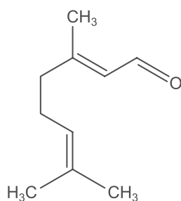
geranial
