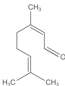
neral
